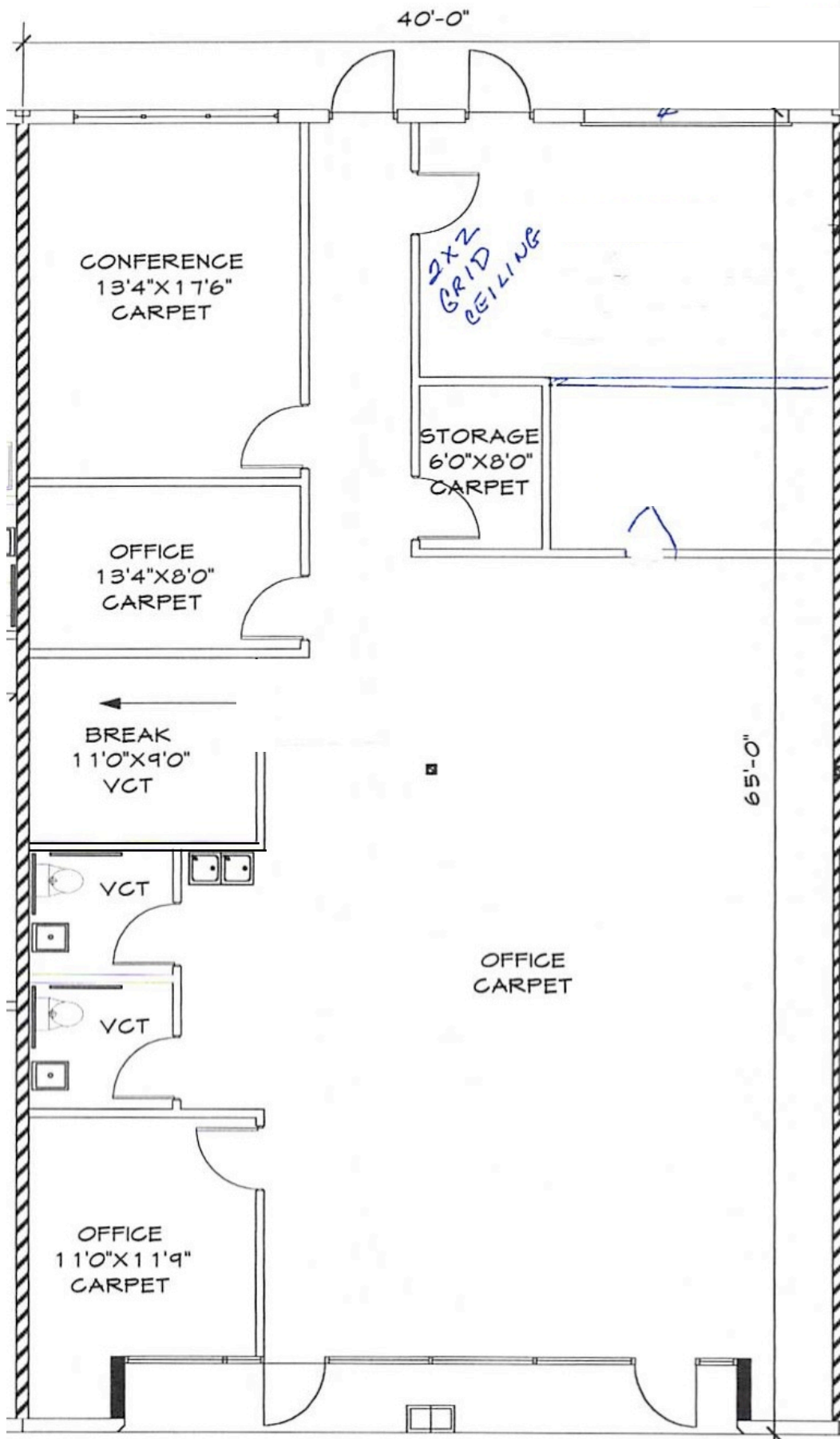
EXHIBIT "A" SUITE 306 2600 SQ. FT. 1/8" = 1'-0"
